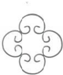
Liscio / Smooth H.215 x L.215 mm Art. 03.706 ≙ 16 x 4
